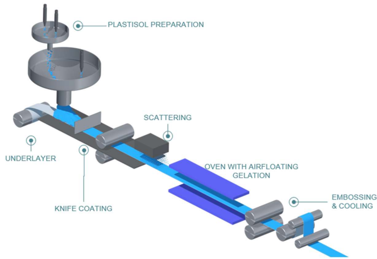
Process flow diagram (coating)
